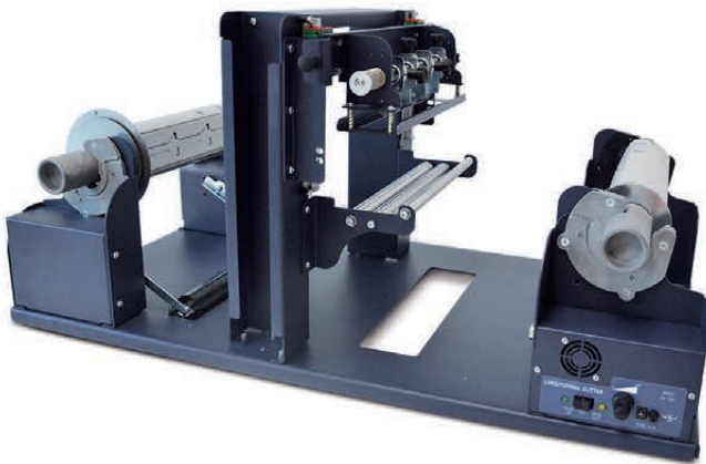
model MCH100SLT25
